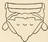
FIG. 19.—HOLOTELSON TUBERCULATUS. ABDOMEN OF FEMALE. \times 3\frac{1}{2} .
